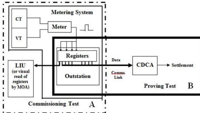
Fig. 1 – Boundaries for Commissioning and Proving Test Activities
